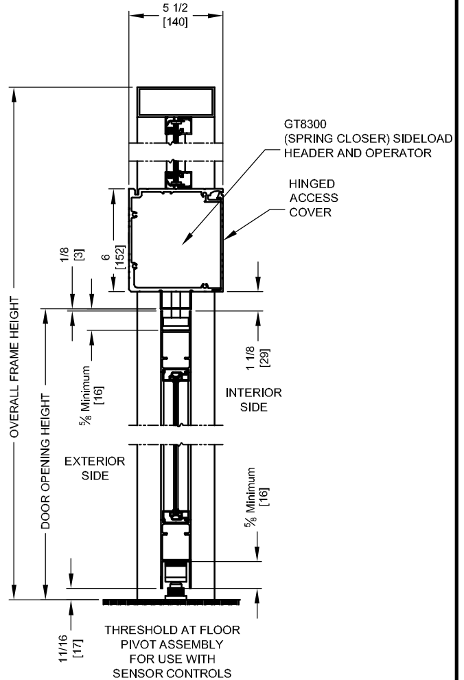
VERTICAL SECTION
