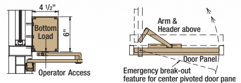
Surface Applied Operator Configurations
