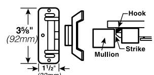
Projection 1 9/16" (21mm)
